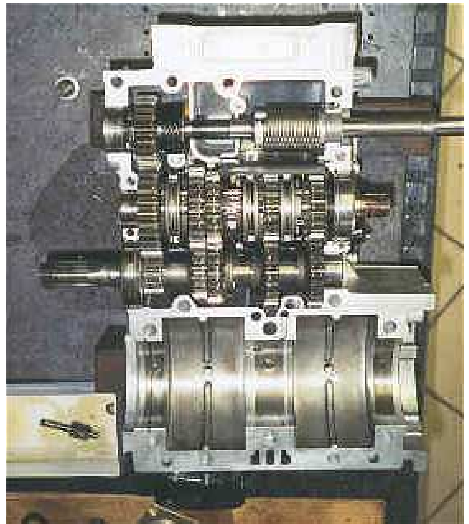
500 gearbox
